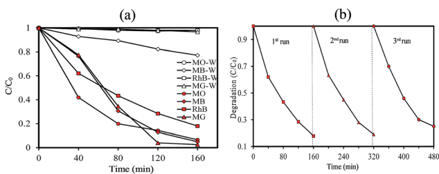
Fig. 5 (a) The photocatalytic degradation of MG, RhB, MB, and MO solution ( 20 \text{ mg L}^{-1} ) in the absence and in the presence of \text{WO}_x/\text{Cs}_y\text{WO}_3 composite, and (b) recycle experiment in the photocatalytic degradation of RhB in the presence of \text{WO}_x/\text{Cs}_y\text{WO}_3 composite under visible light irradiation (LED 30 W).
