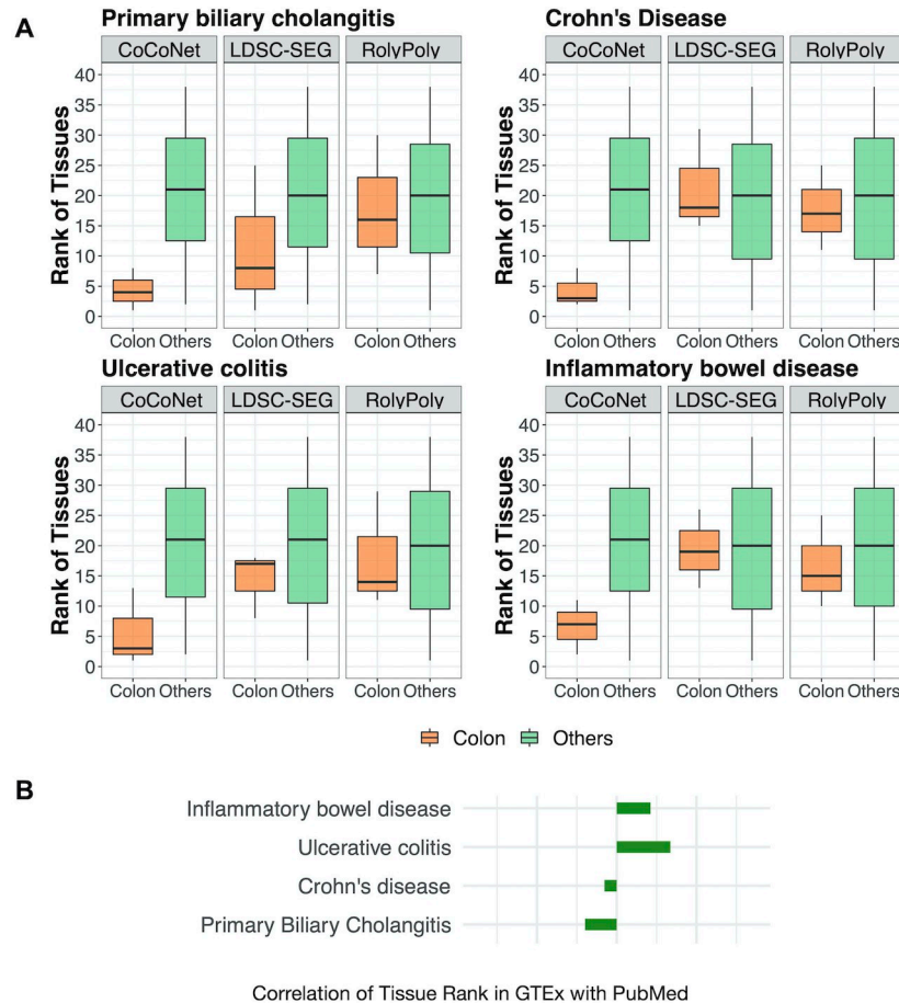
Fig 4. Comparison of tissue rankings by CoCoNet, LDSC-SEG, and RolyPoly for four autoimmune traits. (A): For each of the four autoimmune diseases, we plotted the rank (y-axis) of three colon tissues (colored orange; including colon sigmoid, colon transverse, and intestine terminal ileum) and the rank of the remaining 35 tissues (colored green) in separate boxplots. The rank of colon tissues obtained using CoCoNet is often lower than that of the non-colon tissues (first column in each panel) is often more pronounced than that obtained by either LDSC-SEG (second column) or RolyPoly (third column) for the four autoimmune diseases. (B): We compared the ranking of tissues obtained by CoCoNet with that obtained by PubMed search for 4 autoimmune traits, in the bulk RNAseq data. The CoCoNet and PubMed search results are positively correlated with each other for two traits.
