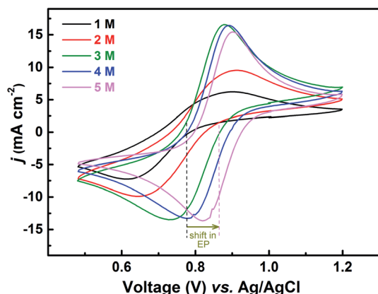
Fig. 8 CVs recorded on carbon-modified GCE at 20 \text{ mV s}^{-1} scan rate in equimolar ( 0.2 \text{ M} ) solution of \text{V}^{4+} and \text{V}^{5+} in \text{H}_2\text{SO}_4 electrolyte of different concentrations. The dotted lines show the shift in EP with supporting electrolyte ( \text{H}_2\text{SO}_4 ) concentration.
