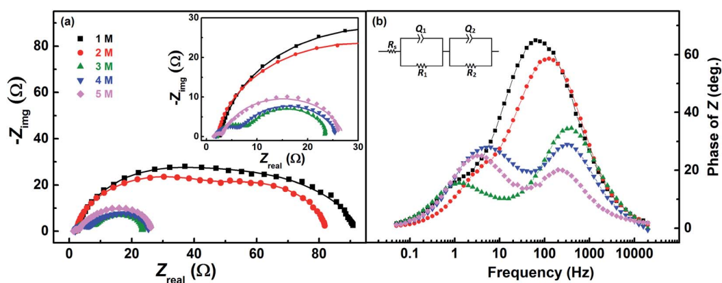
Fig. 9 (a) EIS recorded at EP on carbon-modified GCE with 1600 \text{ rpm} in equimolar ( 0.2 \text{ M} ) concentration \text{V}^{4+} and \text{V}^{5+} in \text{H}_2\text{SO}_4 electrolyte of different concentrations. The corresponding Bode phase plots are shown in (b), along with the equivalent circuit (inset). The symbols and solid lines show the experimental and the fitted data, respectively.
