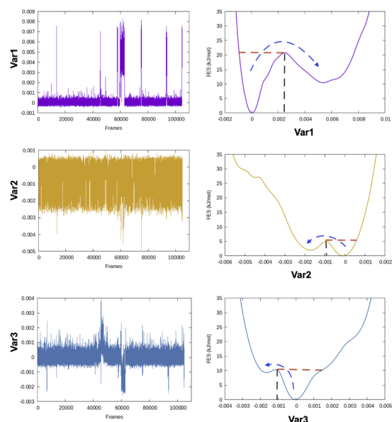
Fig. 2 Fluctuation of three different variables and their corresponding free energy surfaces highlighting the differences in free energy barrier. One can see that the barrier along Var1 is significantly higher compared to other two variables. Heuristically if one has to choose an optimum CV from these three variables, Var1 will be the CV of choice.
