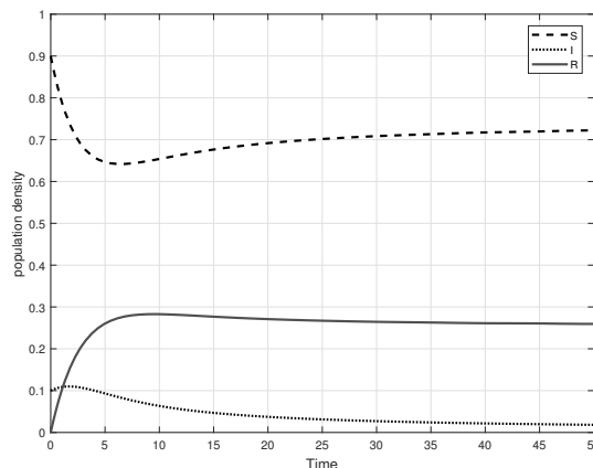
Fig. 3. Point P_1 unstable.
