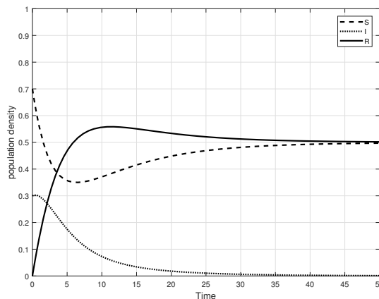
Fig. 4. Stability of P_1 considering R_v < 1 .
