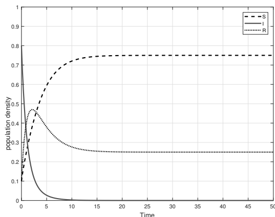
Fig. 2. Point P_1 stable.
