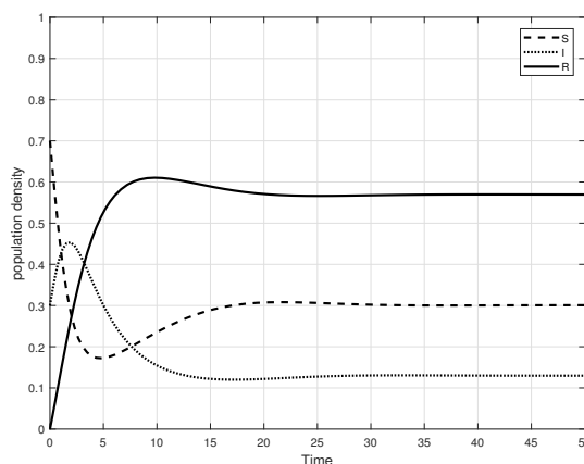
Fig. 5. Stability of P_2 considering R_v > 1 .
