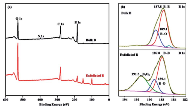
Fig. 8 XPS spectra (survey) (a) and short scan XPS B 1s (b) of bulk B and borophene with few layers obtained by probe ultrasonic assisted solvothermal exfoliation.
