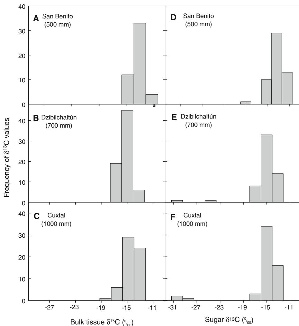
Fig. 2 Frequency of bulk tissue (a–c) and sugar (d–f) \delta^{13}\text{C} values for individuals of 12 CAM species in the coastal dune of San Benito (a, d) and the tropical dry deciduous forests of Dzibilchaltún (b, e) and Cuxtal (c, f). Each bar represents a 2‰ range of \delta^{13}\text{C}
