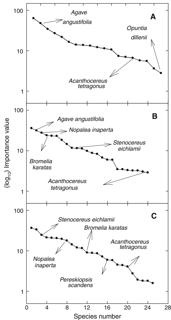
Fig. 1 Relative ecological importance of CAM species in the coastal dune of San Benito (a) and the tropical dry deciduous forests of Dzibilchaltún (b) and Cuxtal (c). Each symbol corresponds to a different species in the communities
