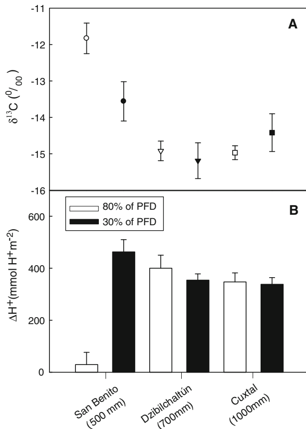
Fig. 5 Values of \delta^{13}\text{C} of sugars (a) and tissue acidity (b) in three populations of Acanthocereus tetragonus in San Benito (circles), Dzibilchaltún (triangles) and Cuxtal (squares) growing at 80% of total daily photon flux density (PFD) (open symbols) or at 30% total PFD (closed symbols) during the rainy season
