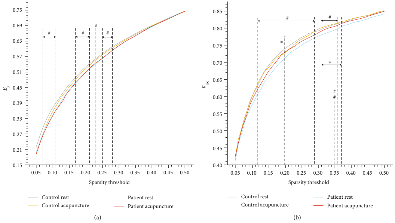
FIGURE 4: Comparison of the global ( E_g ) and local ( E_{loc} ) efficiency at a sparsity range of 0.05-0.50. (a) The stroke patients showed a decline in the global efficiency relative to the healthy controls at certain sparsity ( Sp = 0.07 - 0.11, 0.17 - 0.21, 0.23, 0.25 - 0.28 ). (b) The patients exhibited a conspicuous damage on the local efficiency than the healthy controls ( Sp = 0.12 - 0.29, 0.31 - 0.36 ), while acupuncture intervention showed distinct alteration on the local efficiency of the stroke patients ( Sp = 0.19, 0.20, 0.31 - 0.37 ). \#p < 0.05 , \#\#p < 0.01 (stroke patients vs. healthy controls, in the resting state); *p < 0.05 (resting state vs. postacupuncture intervention, in the stroke patients).
