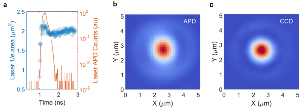
Figure S10. a , On the left axis the laser area expansion in time measured from the scanning APD system. A constant laser area of approximately 2\text{ }\mu\text{m}^2 is observed within the time range of interest. On the right axis the time resolved laser profile is shown. b , Spatial reconstruction of the focused laser image measured from the scanning APD system. c , Focused laser image obtained from the CCD camera (Andor Ixon), consistent with that shown in (b).
