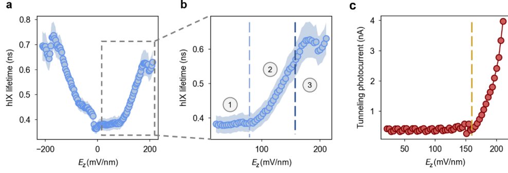
Figure S8. a , Field-dependent lifetime measurements of device B, as reported in Figure 3a in the main text. Here, we focus on the region E_z > 20 mV/nm (dashed grey rectangle). b , For a positive electric field, three main regions are highlighted. Regions 1 ( 20 \text{ mV/nm} < E_z < 80 \text{ mV/nm} ) and 2 ( 80 \text{ mV/nm} < E_z < 160 \text{ mV/nm} ) are characterized by a monotonic increase in \tau_{tot} and correspond to regions of dominating K\Lambda and K\Lambda' transitions, respectively. Instead, region 3 ( E_z > 160 \text{ mV/nm} ) exhibits a sudden drop in \tau_{tot} , which is attributed to the appearance of a nonradiative recombination channel given by the dissociation of hIXs. c , Tunneling photocurrent measured in device B. The rise in signal observed in region 3 is related to the dissociation of hIX at high fields, allowing the extraction of carriers tunneling from WSe 2 to the top and bottom gate electrodes through the hBN layers. Lifetime data are presented as mean values (dots) and corresponding standard deviations (shaded surrounding area).
