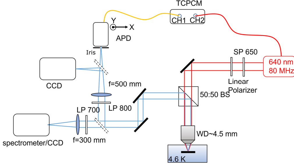
Figure S9. Schematic representation of the complete optical setup for spectroscopic measurements, CCD imaging and scanning APD spatiotemporally-resolved measurements.
