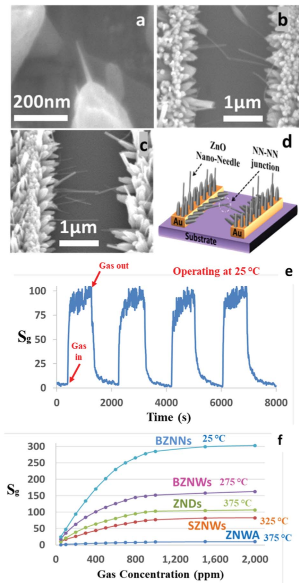
Fig. 8 (a) A high magnification SEM image of a single ZNN, (b) and (c) SEM images of BZNNs, (d) a schematic diagram of the BZNN sensor, (e) response characteristics of the BZNN sensor operated at 25 °C, and (f) sensor response as a function of acetone concentration of the five GSs.
