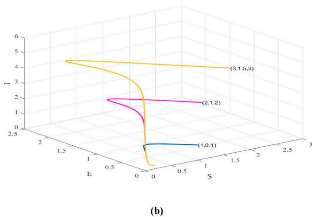
Fig. 8. Shows that global stability of E_1 in S-E-I plane using different initial values ((1,0,1), (2,1,2) and (3,1.5,3) ) and the values of parameters for (a) India (b) Brazil.
