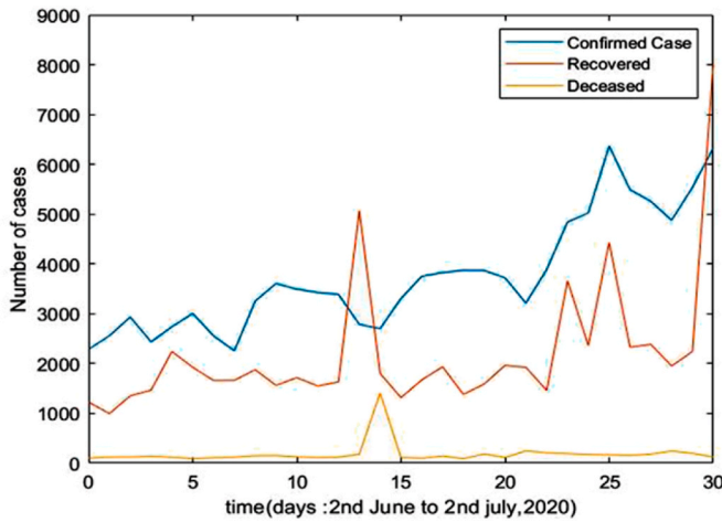
Fig. 2. Confirmed cases, Recovered cases and Deceased cases with respect to time (Days).
