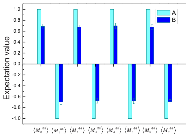
Figure 2 | Experimental results of expectation values of M_k^{\otimes 8} . The settings are measured in 30 minute. Error bars indicate one standard deviation deduced from propagated Poissonian counting statistics of the raw detection events. (A), the theoretical value. (B), the experimental value.
