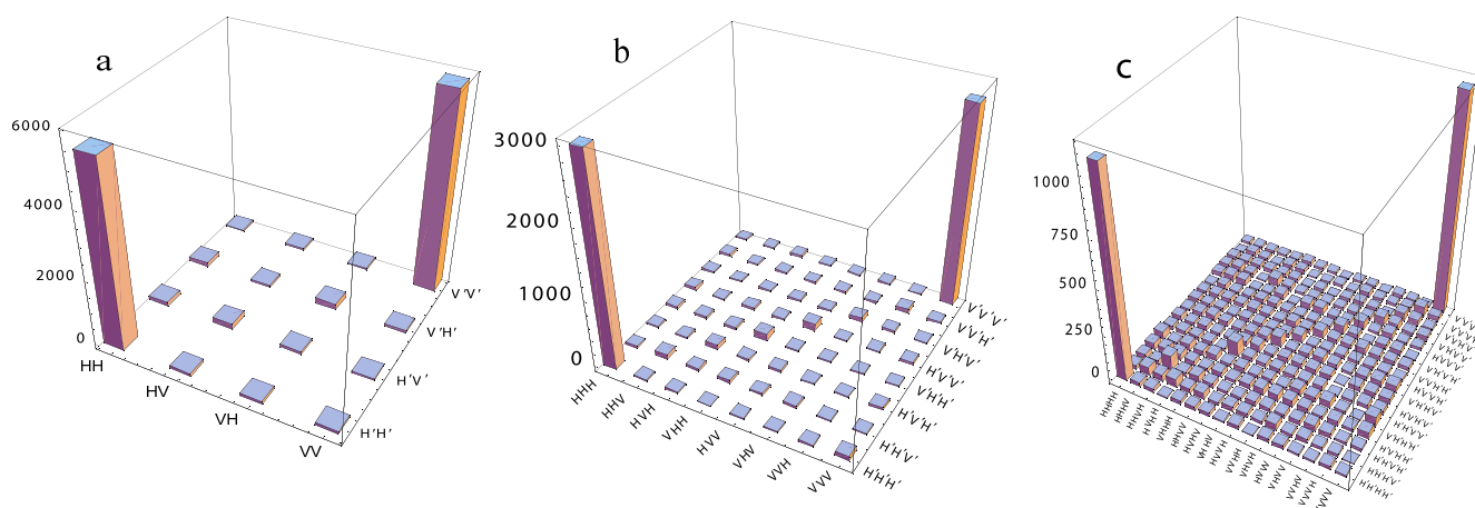
Figure 3 | Experimental results for determination of the four-, six-, and eight-qubit GHZ states. (a), (b), and (c), Coincidence counts obtained in the the |H\rangle/|V\rangle basis ( |H'\rangle/|V'\rangle ) basis, accumulated for 600 s, 900 s, and 1800 s for four-(a), six- (b), and eight-qubit (c) state respectively.
