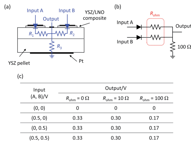
Fig. 6 (a) Schematic picture of the ionic OR gate composed of the YSZ/LNO heterojunction and corresponding equivalent circuit. (b) The model OR gate used in the circuit response simulation. R_{\text{ohm}} represents the ohmic resistance along the lateral direction of the substrate. (c) Electric responses of the model OR gate with different R_{\text{ohm}} .
