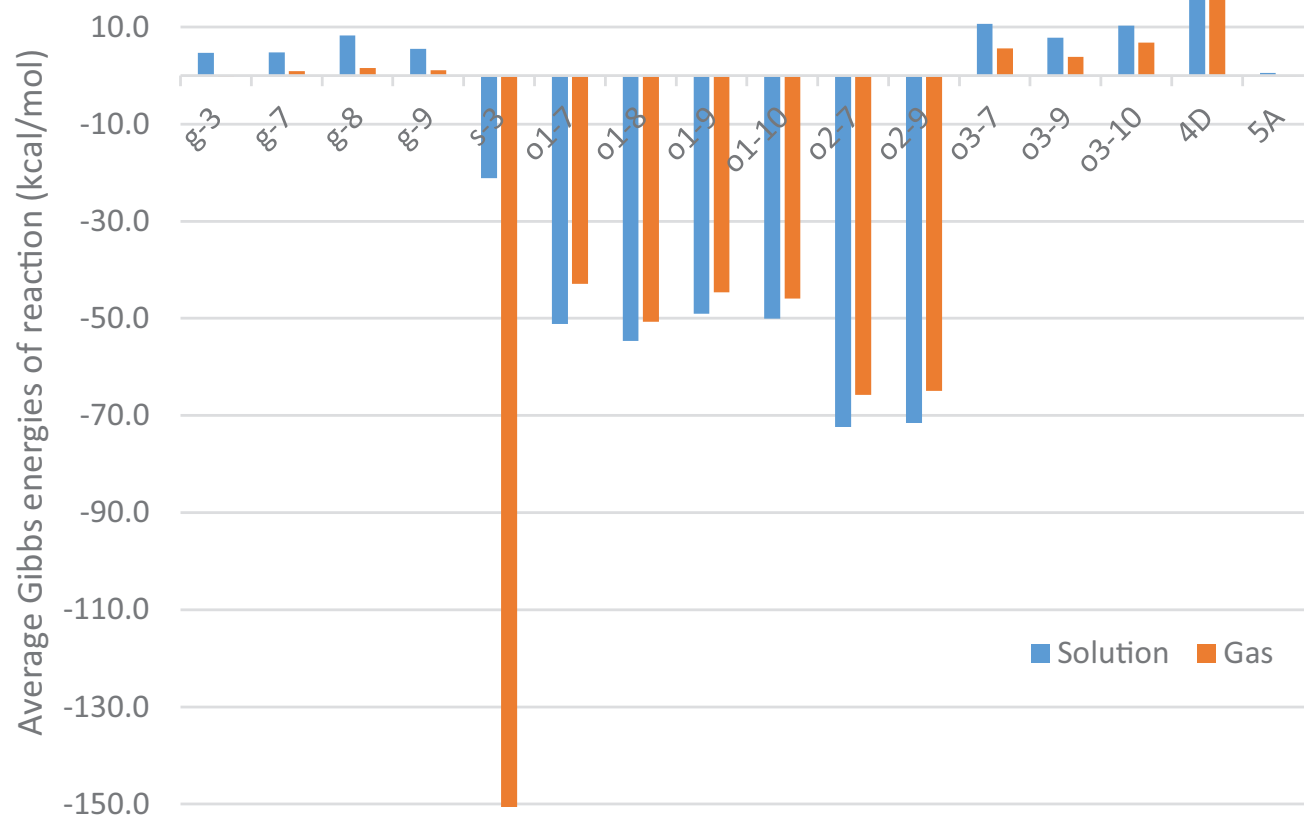
Fig 4. Average Gibbs energies of reaction in the gas phase and in solution for various reactions. Energies were obtained at the B3LYP/6-311++G(d,p) level of theory for each reaction: (o1) oxidation from alkane to alcohol, (o2) oxidation from aldehyde to carboxylic acid, (o3) oxidation from alcohol to aldehyde, (4D) dehydration or four-membered ring formation, (5A) aldol reaction or five-membered ring formation, (g) conjugation with glucuronic acid and (s) conjugation with sulfate at five different positions of (-)-menthol. Representative reactions of each type are shown in Fig 3.
