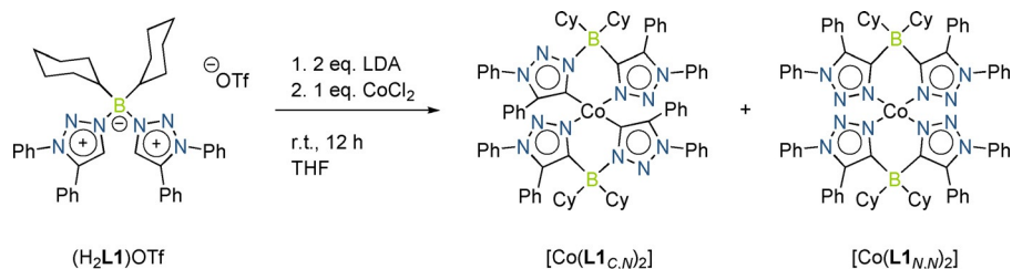
Scheme 2. Synthetic approach for the complexes [Co(L1_{C,N})_2] and [Co(L1_{N,N})_2] .
