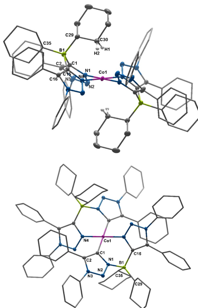
Figure 3. ORTEP representation of [\text{Co}(\text{L1}_{N,N})_2] (top) and [\text{Co}(\text{L1}_{C,N})_2] (bottom). [74] ellipsoids drawn at 50% probability. Solvent molecules and H-atoms omitted (except agostic-interacting \text{CH}_2 groups) for clarity. (For selected bond lengths and angles see supporting information Tables S5 and S6)
