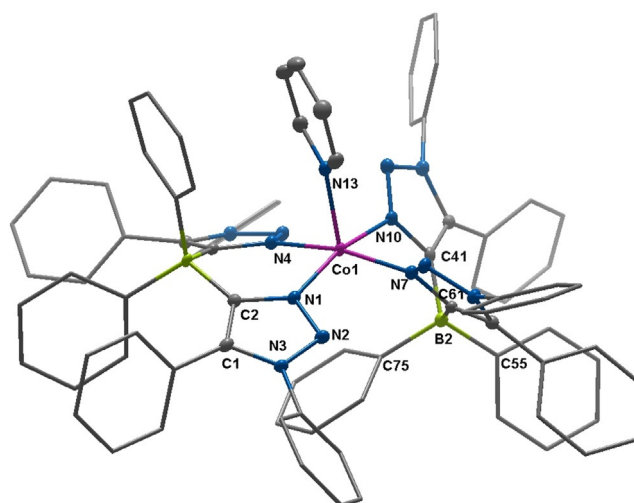
Figure 6. ORTEP representation of [\text{Co}(\mathbf{L2}_{N,N})_2\text{py}]^{[74]} ellipsoids drawn at 50% probability. Solvent molecules and H-atoms omitted for clarity. (For selected bond lengths and angles see supporting information Table S8)
