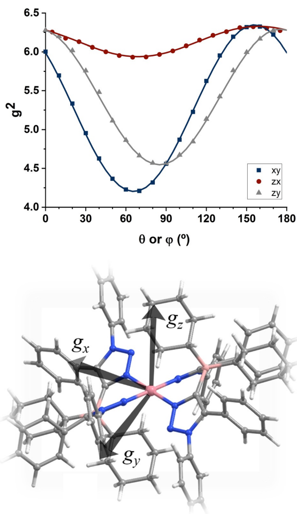
Figure 4. Angular variation of the crystal g^2 -value in three orthogonal planes in the experimental xyz coordinate system, and orientation of the principal axes of the \mathbf{g} -matrix in the molecular coordinate frame.
