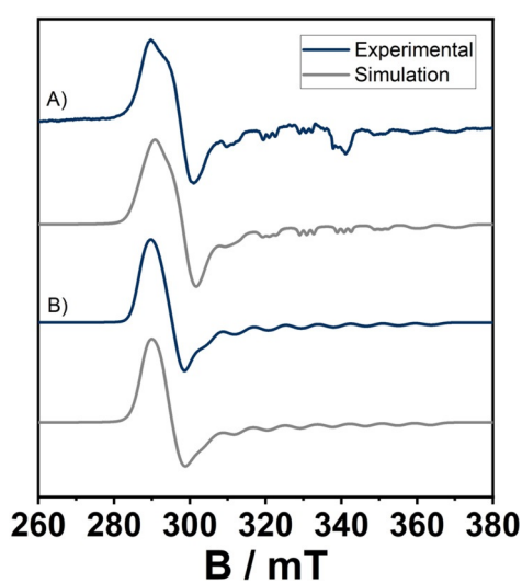
Figure 7. EPR spectra of A) [\text{Co}(\mathbf{L2}_{N,N})_2] in DCM with an excess of pyridine at 100 K. and B) isolated [\text{Co}(\mathbf{L2}_{N,N})_2\text{py}] as a powder at 100 K.
