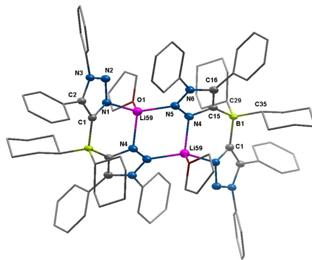
Figure 2. ORTEP representation of [Li(L1_{N,N})_2]^{[74]} ellipsoids drawn at 50% probability. Solvent molecules and H-atoms omitted for clarity. (For selected bond lengths and angles see supporting information Table S9)
