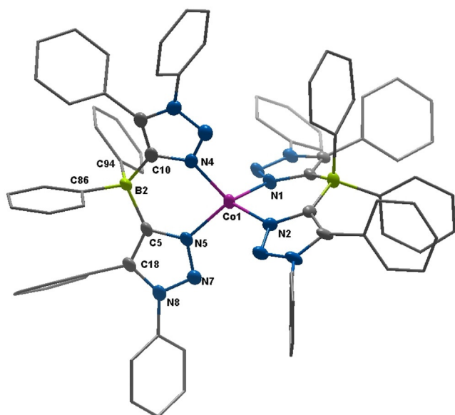
Figure 5. ORTEP representation of [\text{Co}(\mathbf{L2}_{N,N})_2]^{[74]} ellipsoids drawn at 50% probability. Solvent molecules and H-atoms omitted for clarity. (For selected bond lengths and angles see supporting information Table S7)
