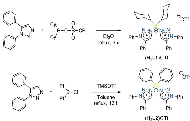
Scheme 1. Synthetic approach for top: (H_2L1)OTf and bottom: (H_2L2)OTf .
