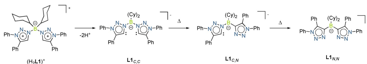
Scheme 3. Deprotonation and isomerization of (\text{H}_2\text{L1})\text{OTf} .
