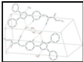
Fig. 2. Part view of the crystal structure, showing hydrogen bonds indicated by dashed lines. Hydrogen atoms not involved in H-bonds have been omitted for clarity.
