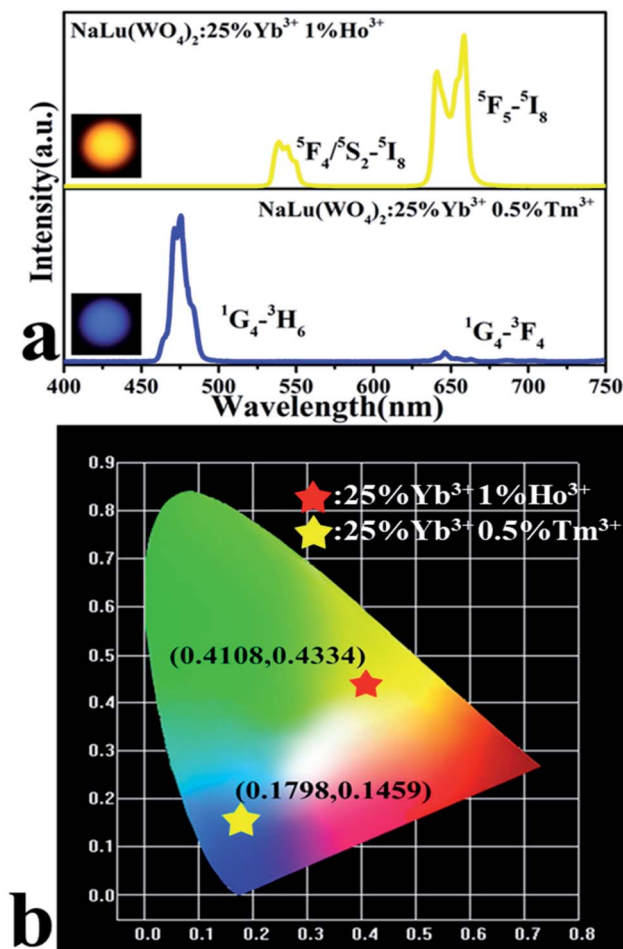
Fig. 4 (a) UC emission spectra and the corresponding luminescence photos of the NaLu(WO 4 ) 2 :25%Yb 3+ , 1%Ho 3+ and NaLu(WO 4 ) 2 :25%Yb 3+ , 0.5%Tm 3+ nanocrystals under excitation at 980 nm; (b) the chromaticity coordinates of NaLu(WO 4 ) 2 :25%Yb 3+ , 1%Ho 3+ and NaLu(WO 4 ) 2 :25%Yb 3+ , 0.5%Tm 3+ .
