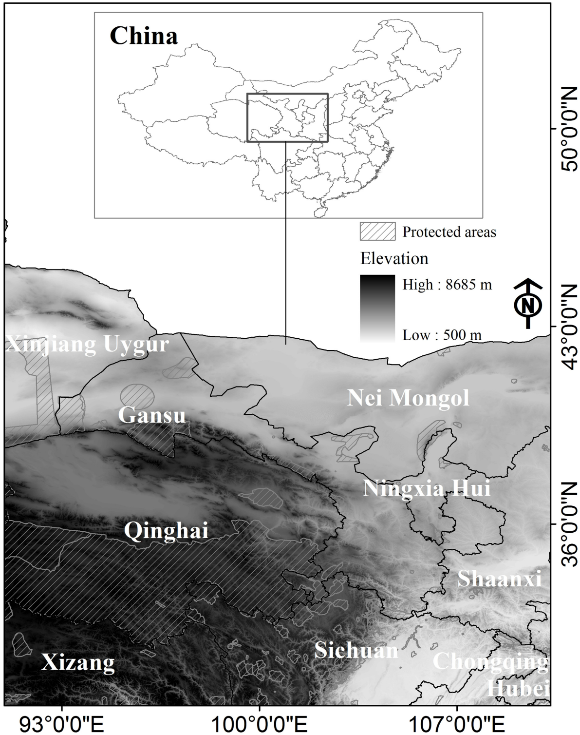
Fig 1. Study areas with elevation ( https://ta.cr.usgs.gov/GMTED2010 ) and protected areas networks [32].
