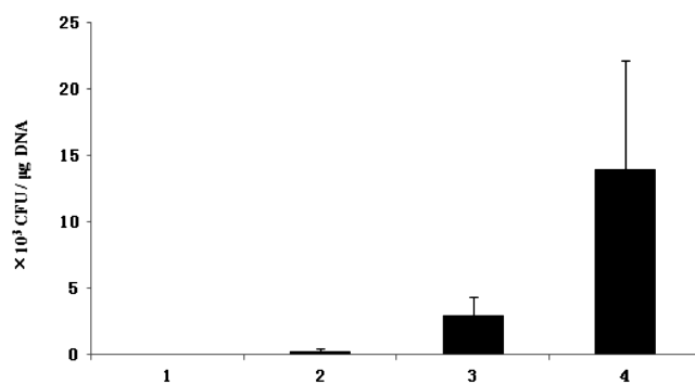
Figure 5. Bleomycin-resistant colonies after inactivation of abrB using cassette lox71-ble-lox66 based PCR products: 1. dsDNA; 2. ssDNA complementary to the leading strand; 3. ssDNA complementary to the lagging strand; 4. ssDNA complementary to the lagging strand with four consecutive phosphorothioated bonds at the 5'-end.
