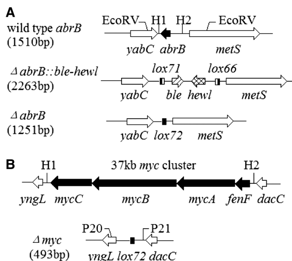
Figure 4. Structure and verification of gene mutation. (A) abrB mutation, the sizes in the brackets indicate the DNA lengths between the two EcoRV restriction sites flanking abrB . (No EcoRV site exists in cassette lox71-ble-hewl-lox66 .) (B) Deletion of myc cluster, the size in the bracket indicates the length of the predicted PCR test product.
