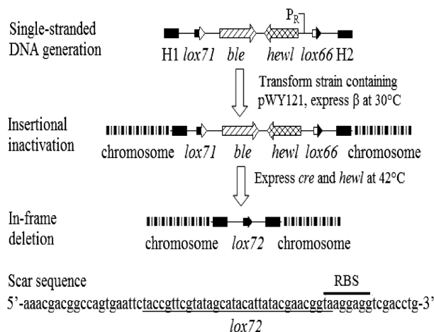
Figure 2. Gene disruption strategy. H1 and H2 refer to the homology extensions. Scar sequence indicates the 69 bp DNA region remained after Cre-mediated excision of the disruption cassette, lox sites and RBS (ribosome binding site) are marked.
