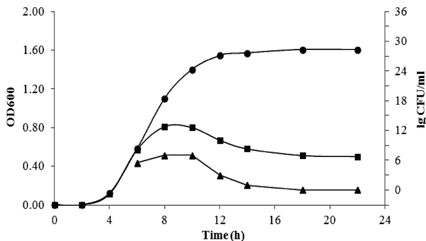
Figure 3. Viability profile of B. subtilis ATCC6633 wild-type and abrB::ble-hewl mutant AL135, both contain pWY121. Incubation temperature was shifted from 30°C to 42°C when the OD600 reached 0.6. Growth curves of wild-type (filled circle) and mutant AL135 (filled square) and logs of AL135 colony forming units (lg CFU/ml) were plotted against time (filled triangle).
