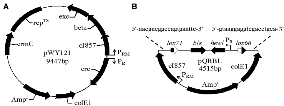
Figure 1. Plasmids used for gene disruptions in B. subtilis . (A) Recombinase genes ( beta and cre ) were cloned into pGE194, with a temperature-sensitive replicon ( rep TS ) and erythromycin resistance gene ( ermC ). Lambda beta and exo were fused downstream of cI857 , under control of P_{RM} , and cre was driven by P_R . (B) A disruption cassette was cloned into pMD19 carrying cI857 to generate pQRBL, the disruption cassette contains bleomycin resistance gene ( ble ), hen egg white lysozyme ( hewI ) encoding gene under control of promoter P_R and lox71/lox66 site at each extremity. Priming sequences for PCR amplification were indicated.
