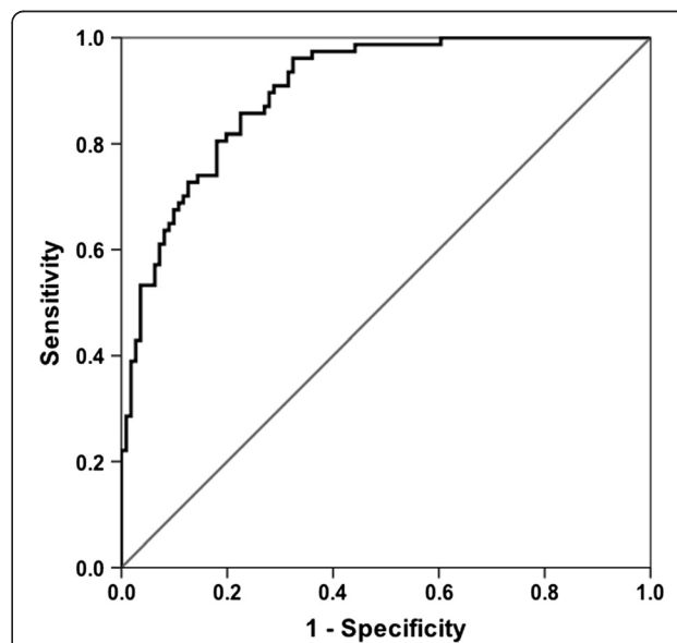
Figure 3 Receiver operator characteristics (ROC) of final multi-analyte model. Area Under the Curve (AUC) = 0.901; 95% CI (0.860-0.943).
