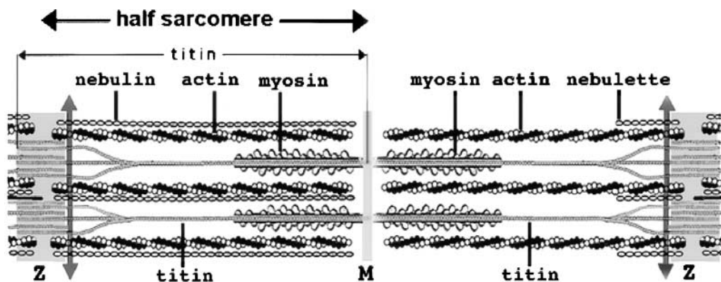
Figure 1. Diagram of a sarcomere bounded by the Z-bands. The left side of the sarcomere represents a half sarcomere found in vertebrate skeletal myofibrils. Note that the nebulin molecules are part of and extend the entire length of the thin filaments. The right side of the sarcomere reflects a half sarcomere in cardiac muscle cells. The smaller nebulin isoform, nebulin, begins within the Z-band and extends only a short distance along the thin filament. Titin is shown with its NH 2 termini from adjacent sarcomeres overlapping in the Z-band. Groups of three titin filaments are shown aligned together in the half sarcomere and overlapping in the M-band with groups of three from the other half sarcomere. The scale of the drawing does not allow the ratio of six titins per half-thick filament or the two nebulin isoforms per actin thin filament to be illustrated. The double-headed arrows indicate the position of the region of titin used as a bait to pull out obscurin. The M-band is the mid-point of the group of aligned thick myosin filaments (A-band) where obscurin binds in cultured neonatal cardiomyocytes and in adult muscles.
