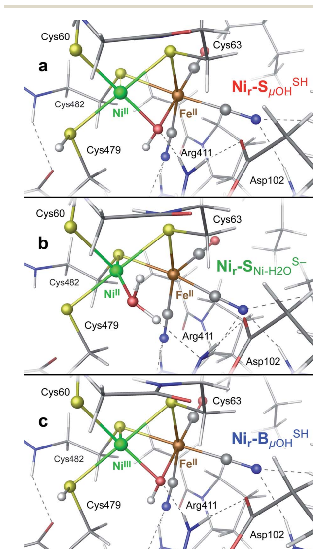
Fig. 3 DFT models: (a) Ni r -S μOH SH of the reduced Ni r -S I state, (b) Ni r -S Ni-H 2 O S- of the reduced Ni r -S II state, and (c) Ni r -B μOH SH of the oxidized Ni r -B'' state, displaying the [NiFe] cofactor metal ligands and their contacts with the nearby side chains in HoxC. For alternative models and the entire HoxC homology model employed, see Fig. S4–S10.†
