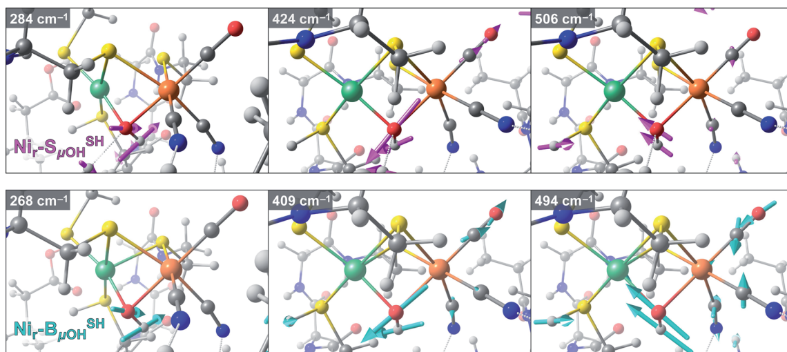
Fig. 7 Arrow-style representation of important Fe/Ni– \mu\text{OH} vibrational modes from representative DFT models for the Ni r -S _{\text{I}} (model Ni r -S _{\mu\text{OH}}^{\text{SH}} , top) and Ni r -B'' (model Ni r -B _{\mu\text{OH}}^{\text{SH}} , bottom) states. The corresponding vibrational energies ( \text{cm}^{-1} ) are indicated in the top left of each panel. Left to right: Ni– \mu\text{OH} -Fe wagging, Fe– \mu\text{OH} stretching, and Ni– \mu\text{OH} stretching modes. The stick-style mode intensities relevant to the interpretation of the ^{57}\text{Fe} -PVDOS spectra are marked in Fig. S18b and S19b–d.† Animations of these and other normal modes are available as part of the ESI.†
