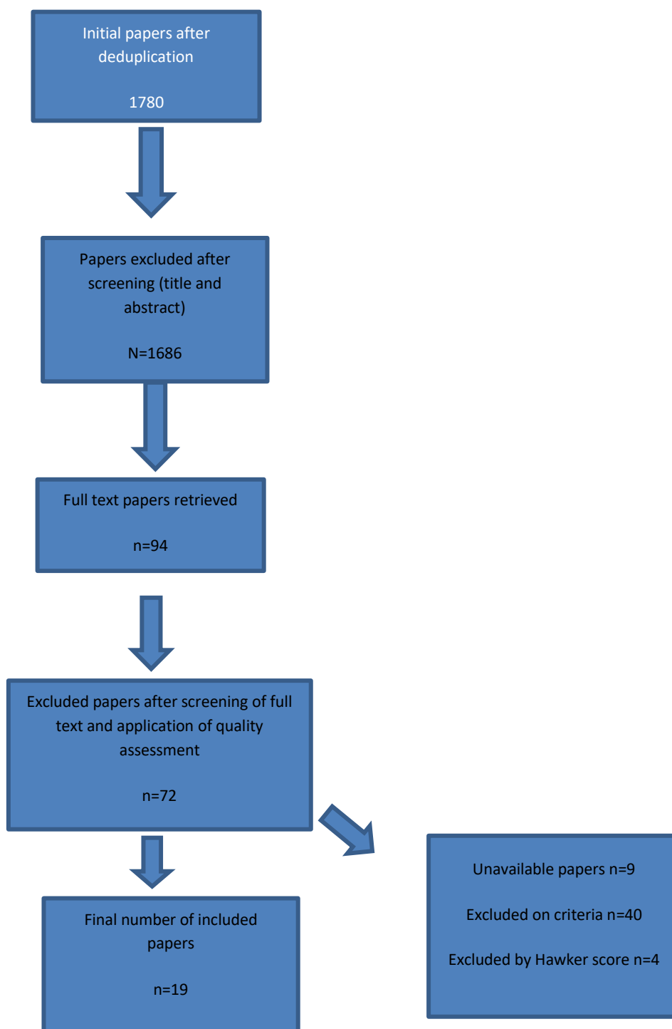
Figure 1. Prisma Diagram.
