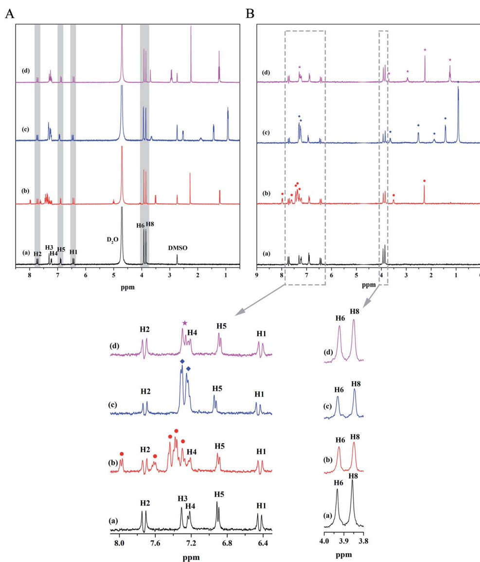
Fig. 5 (A) ^1\text{H} NMR spectra of: (a) MF; (b) MF–warfarin sodium (1 : 1); (c) MF–ibuprofen (1 : 1); (d) MF–lidocaine (1 : 1). C_{\text{MF}} = 1.3 \times 10^{-3} \text{ M} . (B) STD-NMR spectra of the site-marker-displacement experiments: (a) HSA–MF (1 : 130); (b) HSA–MF–warfarin sodium (1 : 130 : 130); (c) HSA–MF–ibuprofen (1 : 130 : 130); (d) HSA–MF–lidocaine (1 : 130 : 130). C_{\text{HSA}} = 10 \times 10^{-6} \text{ M} . The bottom figures show the magnified view of the portion of the corresponding dashed box. ★: lidocaine, ◆: ibuprofen, ●: warfarin sodium.
