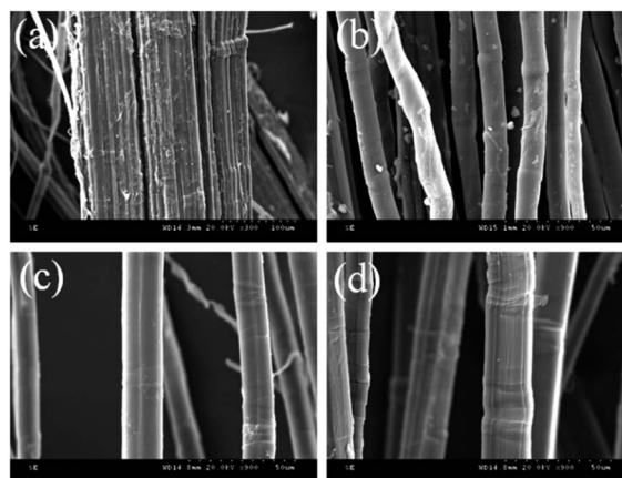
Fig. 7 SEM image of the hemp fiber: (a) untreated hemp fiber, (b) traditional alkali degumming hemp fiber, (c) traditional Fenton degumming hemp fiber, and (d) Fenton- \text{MnFe}_2\text{O}_4 degumming hemp fiber.
