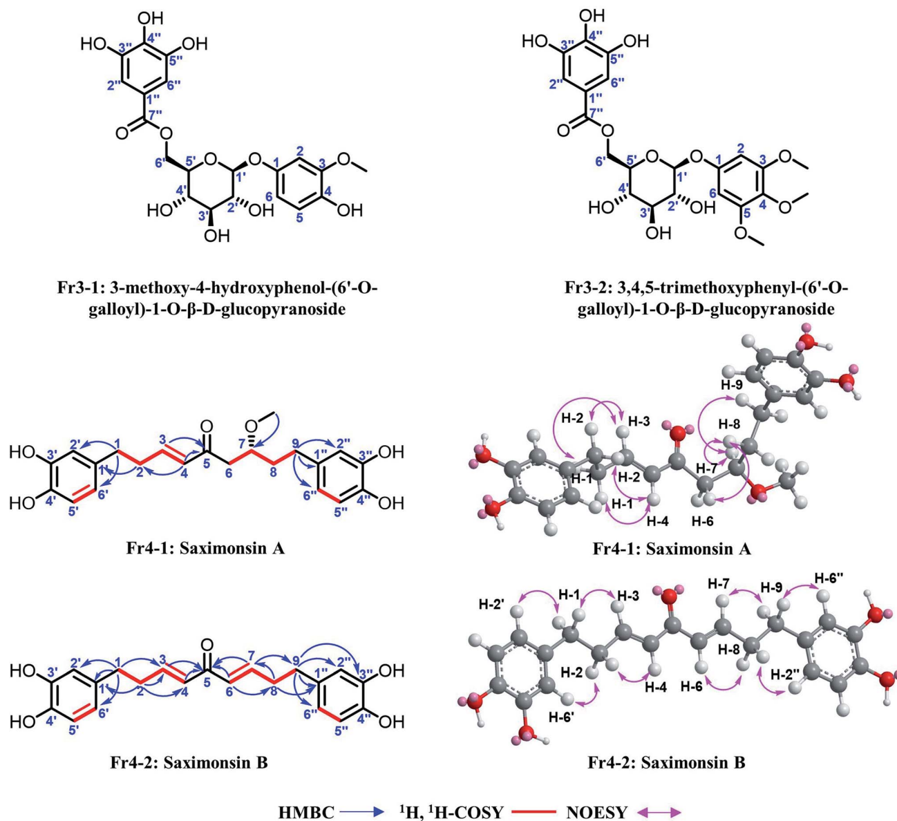
Fig. 6 Chemical structures and the HMBC, 1 H, 1 H-COSY and NOESY correlations of the isolated DPPH inhibitors.
