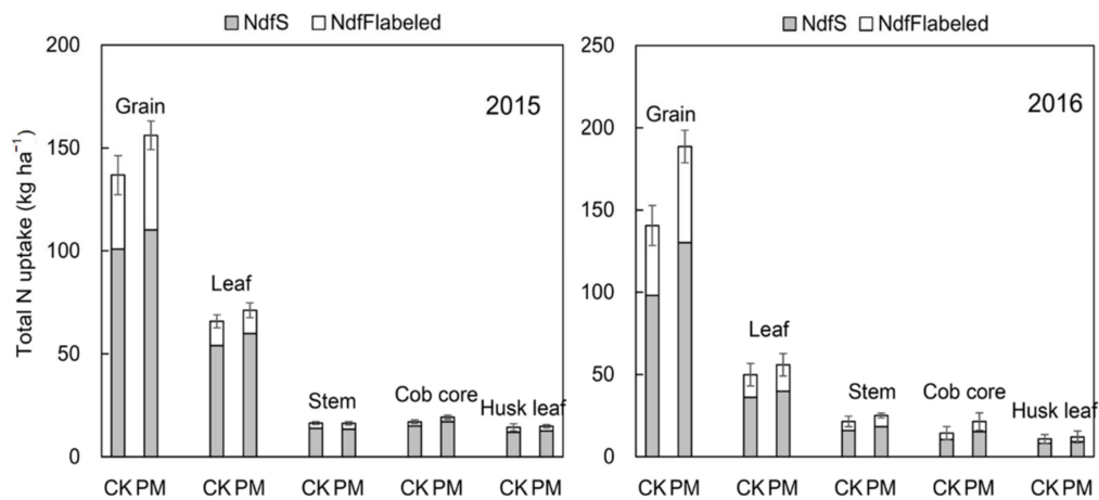
Figure 4. Maize dry matter biomass, total N uptake, N derived from the soil (NdfS) and fertilizer (NdfFlabeled), N derived from labeled-urea fertilizer (NdfFlabeled), as affected by plastic mulch at harvest in 2015–2016.
