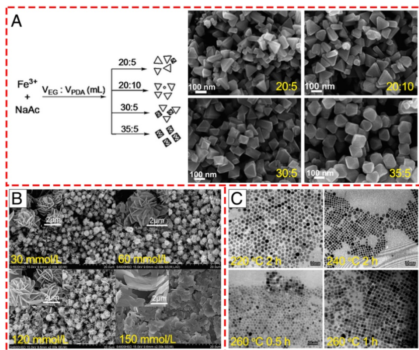
Figure 3. Controlled synthesis of different shapes of IONPs via varying the reaction conditions. (A) Varying the solvent component ratio. Reproduced with permission from [41], copyright 2010. (B) Controlling the alkaline reaction environment via different concentration of TBAB. Reproduced with permission from [42], copyright 2011. (C) Controlling the reaction temperature and time. Reproduced with permission from [43], copyright 2010.
