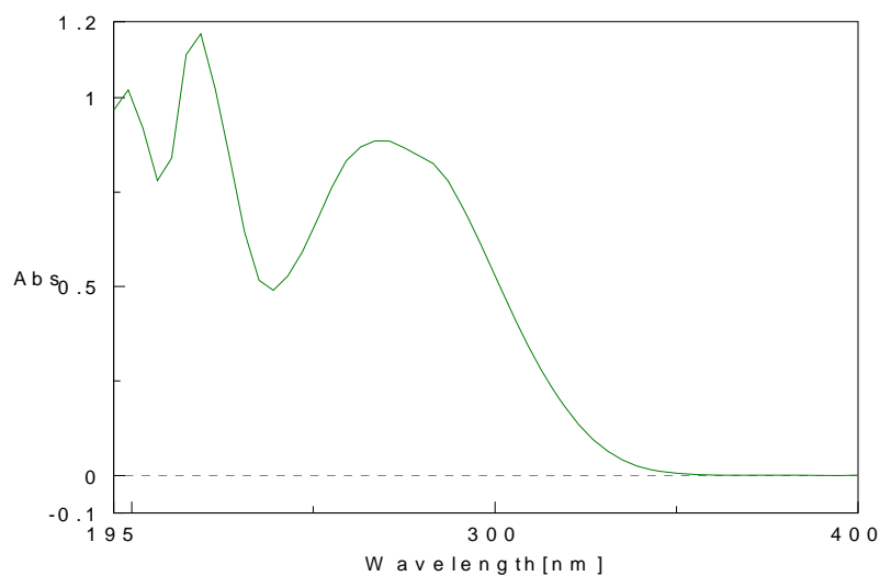
UV spectrum
