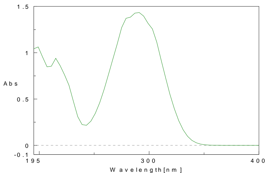
UV spectrum
