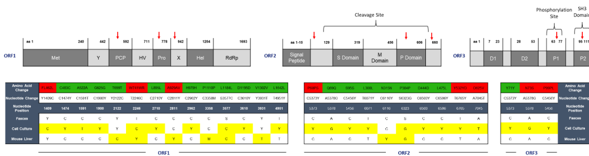
Figure 3. HEV adapts to in vitro culture but shows limited mutagenesis in the humanized mouse model. Genomic differences after in vitro and in vivo passage of HEV derived from HEV0069 feces are depicted per ORF. The HEV0069 feces isolate is used as reference sequence and the nucleotide and amino acid sequence differences are highlighted in yellow and red, respectively. nt, nucleotide; aa, amino acid; ORF, open reading frame; Green, no change in amino acid sequence; Red, change in amino acid sequence; Yellow, nucleotide differences with respect to feces nucleotide sequence. Nucleotide abbreviations; M = A,C; S = G,C; W = A,T; Y = T,C. HEV0069 sequence is relative to HEV wbGER27 (GenBank accession number: FJ705359).
