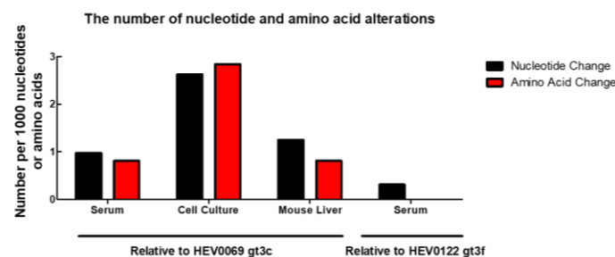
Figure 4. Frequency of alterations was highest after in vitro cell culture. The number of mutations in isolates obtained from serum, cell culture, and human liver chimeric mouse liver relative to the sequence derived from the feces isolate. The number of variations was divided by the total sequence length of the genome or the expected protein sequence length and then normalized to 1000 nucleotides or amino acids.
