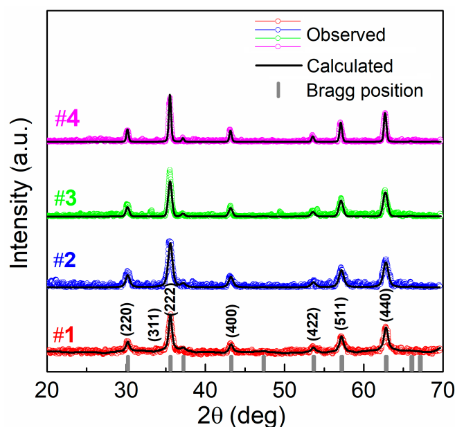
Figure 1. X-ray Diffraction (XRD) spectra of the four synthesized samples of \text{Fe}_3\text{O}_4 nanoparticles (NPs), analyzed by the Rietveld refinement method.
