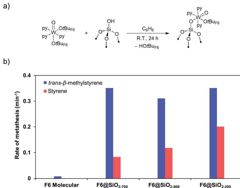
Fig. 6 (a) Preparation of well-defined silica-supported W(IV) oxo species. (b) Rates of metathesis of trans\text{-}\beta\text{-methylstyrene} (blue) and styrene (red) catalysed by W(IV) oxo species, molecular and supported on silica prepared at different dehydroxylation temperatures. Reprinted with permission from ref. 164. Copyright 2019 American Chemical Society.
