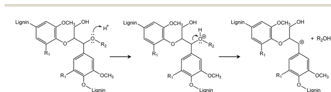
Scheme 1 Formation of carbocation on a representative lignin structure under acidic conditions ( R_1 = \text{H} or \text{OCH}_3 , R_2 = \text{Ar} ). 13
