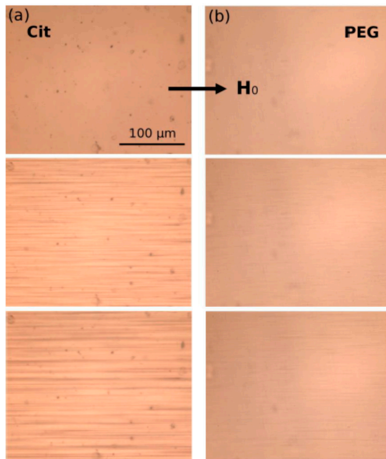
Figure 28. Optical microscopy images of aqueous suspensions of (a) citrated, and (b) PEGylated MNCs in an external uniform DC magnetic field of intensity 13.5 kA/m. Each row corresponds to the elapsed time from the moment of the magnetic field application t = 0 (upper row), 5 and 10 min. (Reprinted from [274] under Open Access license).
