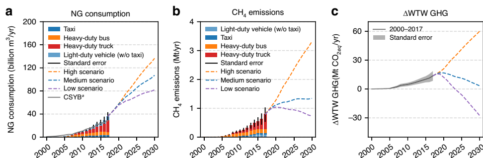
Fig. 4 NG consumption, total CH 4 emissions from NGVs, and changes of WTW GHG emissions of switching to NGVs in China from 2000 to 2030.
