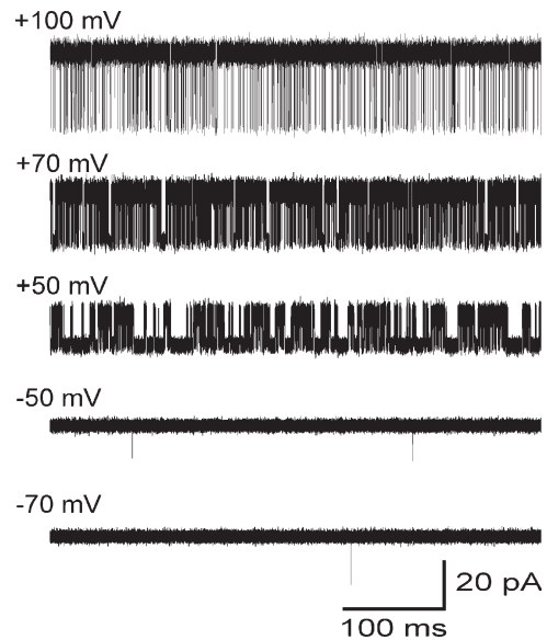
Figure 7. Simulated single-channel currents for Scheme V for BK_B channel DM4 at the indicated voltages with saturating Ca^{2+}_i . The simulated single-channel currents reproduce the kinetic properties of the experimental single-channel currents shown in Fig. 1.
