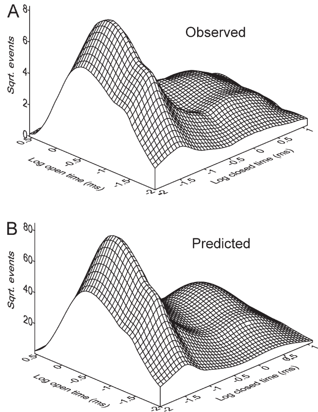
Figure 6. Observed and predicted 2-D dwell-time distributions of open-closed- and closed-open-interval pairs for Scheme V for BK_B channel DM4 at 50 mV with saturating Ca^{2+}_i . Scheme V approximated the 2-D distributions.
