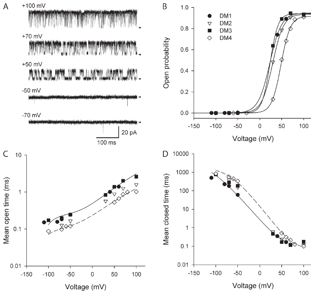
Figure 1. Voltage activation of BK B channels. (A) Representative single-channel currents recorded from a BK B channel (DM4) in saturating 95 μM Ca 2+ i . Arrows indicate the closed channel levels. (B) Plots of Po versus voltage for four separate BK B channels, as indicated. The lines are fits with the Boltzmann equation P_o = P_{o_{max}} / (1 + \exp[(V_{0.5} - V)/b]) , where b is the voltage sensitivity expressed as the voltage change (in millivolts) per e-fold change in Po. The parameters for the lines are given in Table I. (C and D) Voltage dependence of mean open and mean closed times for the same four channels as in B. The lines plot the predicted mean open and closed times for channels DM1 (continuous lines) and DM4 (dashed lines) calculated with Scheme V. A similar superposition of observed and predicted mean open and mean closed times was observed for channels DM2 and DM3. Parameters used in the predictions for channel DM4 in C and D of this figure and in Figs. 4–7 are given in Table S3.
