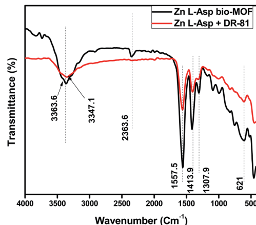
Fig. 13 FTIR spectra of before and after DR-81 dye adsorption.
