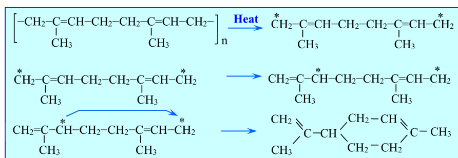
Figure 4. Mechanism of the pyrolytic decomposition of natural rubber (polyisoprene) to propylene and its isomerization into limonene [25].
