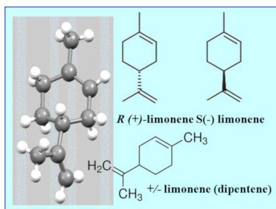
Figure 1. Structural formulas of limonene and its enantiomers.
