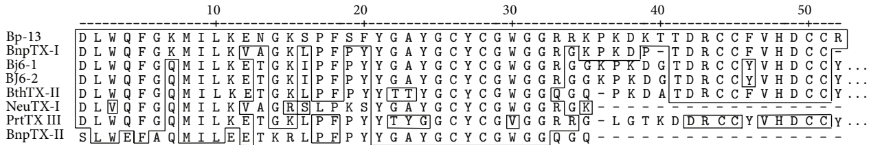
FIGURE 4: The amino acid sequence N-terminal, alignment of Bp-13 with selected PLA 2 sequences obtained from the BLAST protein data bank (PubMed-Medline). PrtTX III from Bothrops pirajai [55], PLA 2 Bj p from Bothrops jararacussu [30], PLA 2 6-1 and PLA 2 6-2 [22] and BthTx-II, bothroptoxin II, from Bothrops jararacussu [56], BnpTX-I and BnpTX-II [32], and NeuTX-I [12].
