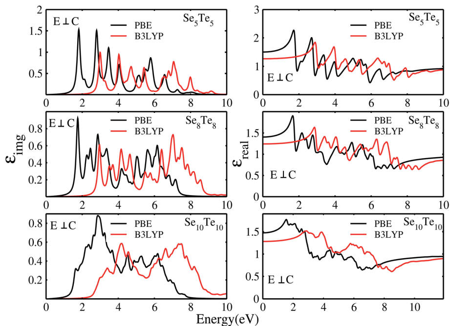
Fig. 12 Dielectric function with PBE and B3LYP hybrid functionals for E ⊥ C.
