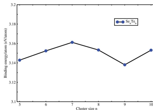
(b) Binding energy/atom as a function of cluster sizes
