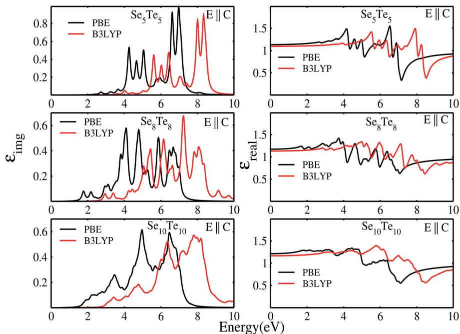
Fig. 13 Dielectric function with PBE and B3LYP hybrid functionals for E || C.
