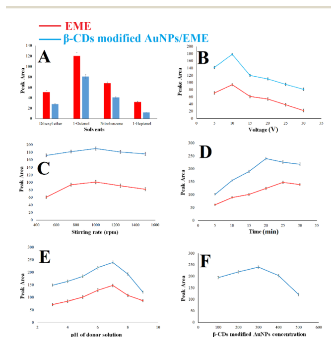
Fig. 4 (A) Effect of the SLM composition on the EME and \beta -CD-modified AuNPs/EME methods; (condition: 100 \text{ng mL}^{-1} of methadone, 750 rpm as the stirring rate, voltage of 15 V, 15 min extraction time, donor solution pH of 7.0, and 300 \mu\text{L} of \beta -CD-modified AuNPs), (B) effect of applied voltage; (condition: 100 \text{ng mL}^{-1} of methadone, 750 rpm as the stirring rate, 15 min extraction time, donor solution pH of 7.0, and 300 \mu\text{L} of \beta -CD-modified AuNPs), (C) effect of stirring rate; (condition: 100 \text{ng mL}^{-1} of methadone, voltage of 10 V, 15 min extraction time, donor solution pH of 7.0, and 300 \mu\text{L} of \beta -CD-modified AuNPs), (D) effect of extraction time; (condition: 100 \text{ng mL}^{-1} of methadone, voltage of 10 V, 1000 rpm as the stirring rate, donor solution pH of 7.0, and 300 \mu\text{L} of \beta -CD-modified AuNPs), (E) effect of donor solution pH; (condition: 100 \text{ng mL}^{-1} of methadone, voltage of 10 V, 1000 rpm as the stirring rate, 20 min extraction time for the \beta -CD-modified AuNPs/EME method and 25 min extraction time for the EME method, and 300 \mu\text{L} of \beta -CD-modified AuNPs). (F) Effect of \beta -CD-modified AuNP concentration; (condition: 100 \text{ng mL}^{-1} of methadone, voltage of 10 V, 1000 rpm as the stirring rate, 20 min extraction time for the \beta -CD-modified AuNPs/EME method and 25 min extraction time for the EME method, and solution pH of 7.0). The red color indicates the EME method parameters, and the blue color indicates the \beta -CD-modified AuNP method.
