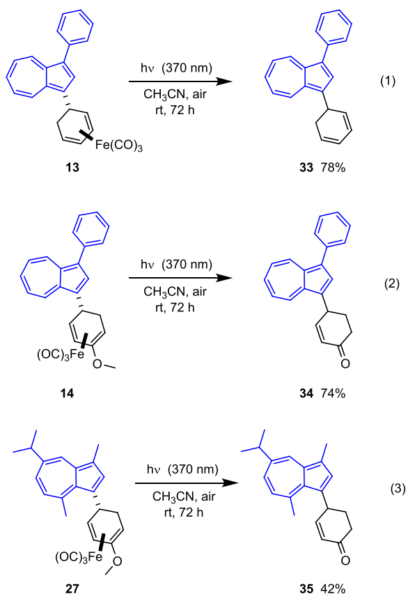
Scheme 7. Photolytic Decomplexation of Addition Products a
