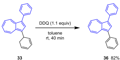
Scheme 8. Aromatization of Free Diene
