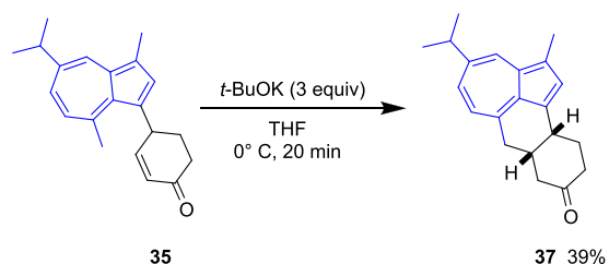
Scheme 9. Base-Mediated Cyclization of Demetallated Guaiazulene Derivative 35 Forming Tetracycle 37 a,b
