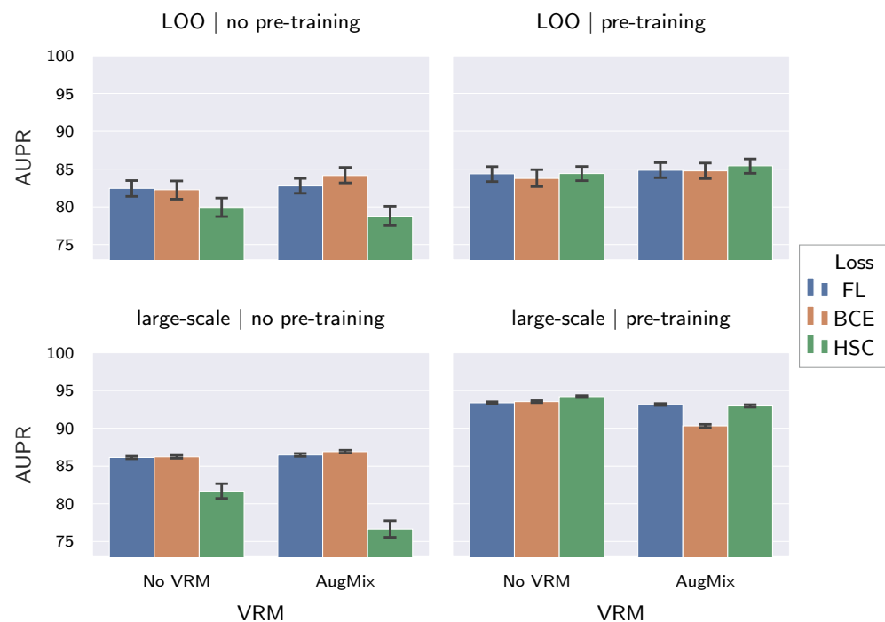
Figure 5. Influence of ImageNet pre-training, loss function and AugMix on the resistance of supervised fabric AD methods to distribution shifts. We show both mean and 95% confidence interval (CI) for the AUPR achieved on the held-out fabrics, as well as on the large-scale dataset.
