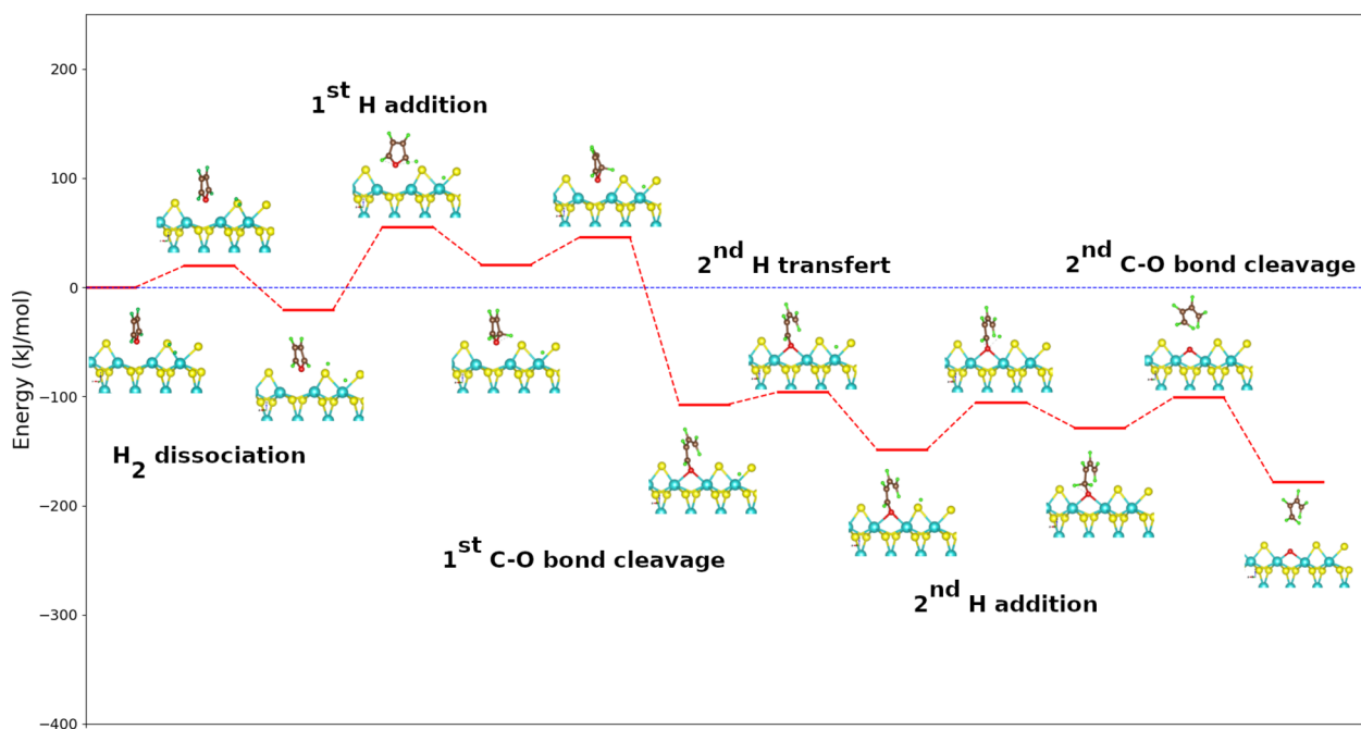
Fig. 2 Energy diagram of the DDO route of furan on the metal edge of MoS 2 surface using the PBE + D2 approximation. For clearer images, please refer to Fig. S6 in the ESI.†
