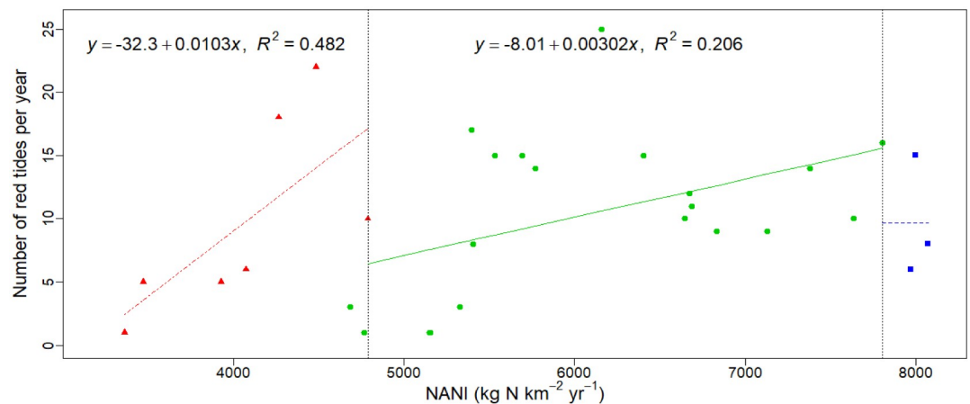
Fig 6. Correlation between NANI and the number of red tides occurring per year in Guangdong coasts between 1986–2015.
