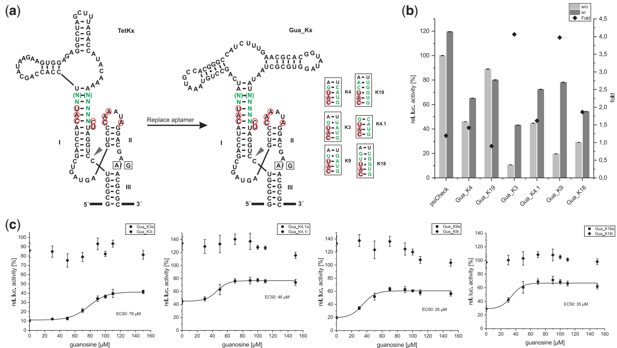
Figure 3. Rational design of guanine-sensing aptazymes in HeLa cells. (a) The tetracycline aptamer in the TetK4/K19 constructs (10) is replaced by the guanine-sensing xpt aptamer (16), while the respective communication module (green) remains identical. Additional tested communication modules (K3, K4.1, K9, K18) are presented as well. Nucleotides involved in the stem I-stem II tertiary interactions of the ribozymes are encircled in red. A ribozyme inactivating A→G mutation is depicted. (b) Dual luciferase assay of the constructs shown in (a). Transfected cells were incubated in the absence or presence of 500 \mu\text{M} guanosine. Experiments were performed in triplicates and error bars represent standard deviation. A psiCheck2 plasmid without aptazyme serves as control. (c) Dose dependency of the Gua_K3, Gua_K4.1, Gua_K9 and Gua_K18 switches. The relative luciferase activity under control of the respective switch and an inactivated variant is shown under varying guanosine concentrations. A sigmoidal fit was used to calculate the EC50-value. Experiments were performed in triplicates and error bars represent standard deviation.
