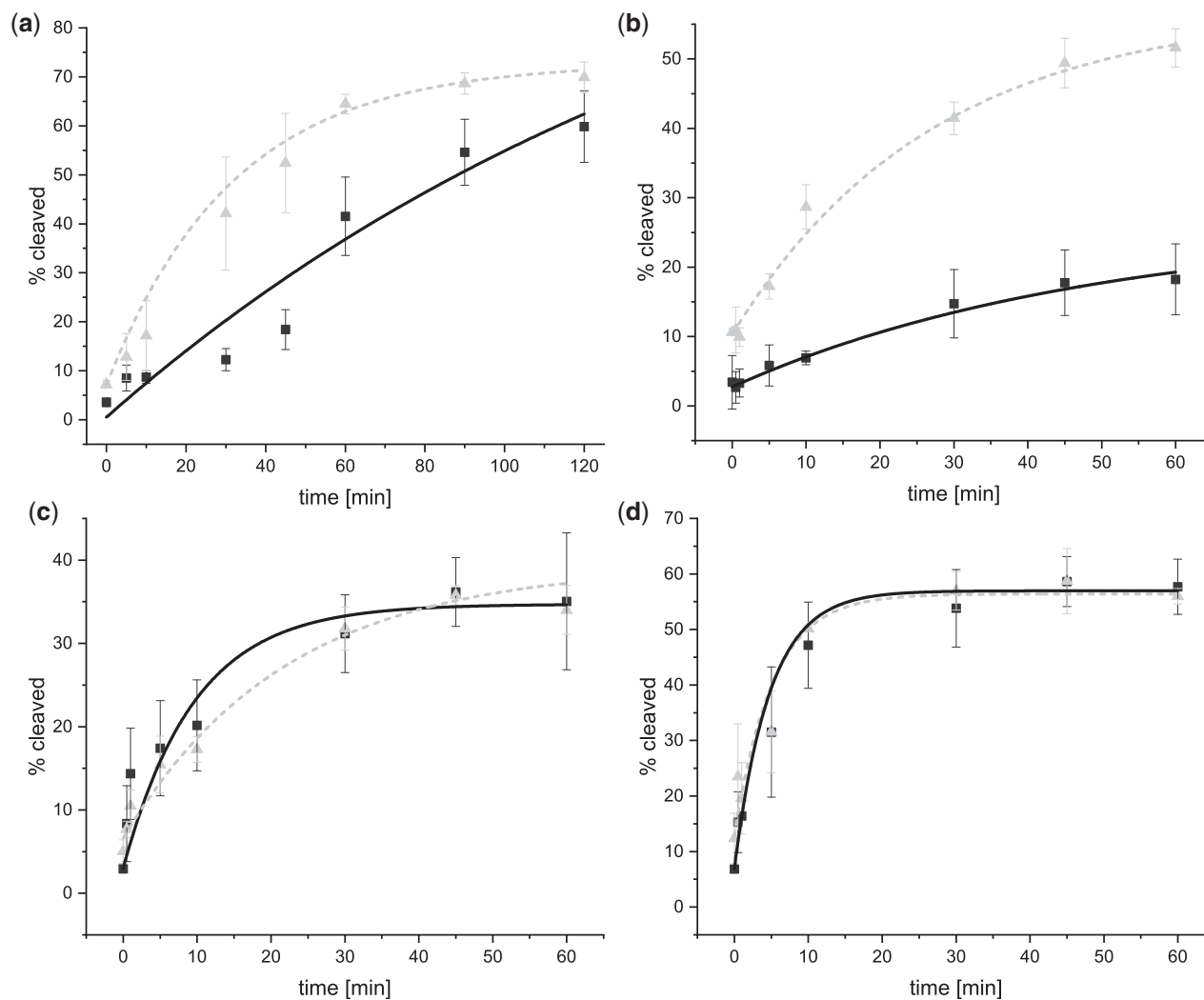
Figure 2. Cleavage activities of aptazyme sequences in vitro . Percentage of cleaved fraction for ON-switches (a) Gua_eco1, (b) Gua_eco2 and OFF-switches (c) Gua_eco3, (d) Gua_eco4 in absence (black line) and presence (grey dashed lines) of guanine.
