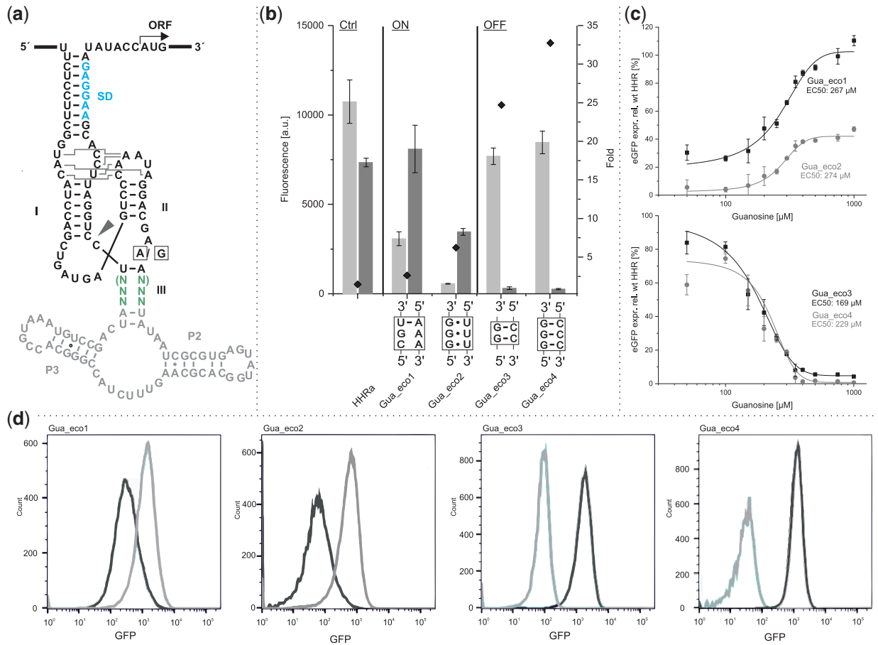
Figure 1. Screening and characterization of guanine-sensing aptazymes in E. coli . (a) A Type I HHR (black) is inserted in the 5' UTR of an eGFP reporter gene. The Shine-Dalgarno (SD, blue) sequence is included in an extended stem I of the ribozyme. The xpt aptamer (light grey) is connected to the HHR via a communication module (green) with either four or six randomized nucleotides. (b) Bulk measurement of selected switches. The communication module of each switch is depicted underneath. An active HHR without aptamer domain served as control. Experiments were performed in triplicates and error bars represent standard deviation. (c) Dose dependency of the switches. The eGFP expression under control of the ON-switches Gua_eco1 and Gua_eco2 or the OFF-switches Gua_eco3 and Gua_eco4 relative to the expression under control of a HHRa is shown under varying guanosine concentrations. A sigmoidal fit was used to calculate EC50-values. Experiments were performed in triplicates and error bars represent standard deviation. (d) Flow cytometry histograms of the eGFP expression under control of the ON-switches Gua_eco1 and Gua_eco2 or OFF-switches Gua_eco3 and Gua_eco4 in absence (black) and presence (grey) of 1 mM guanosine.
