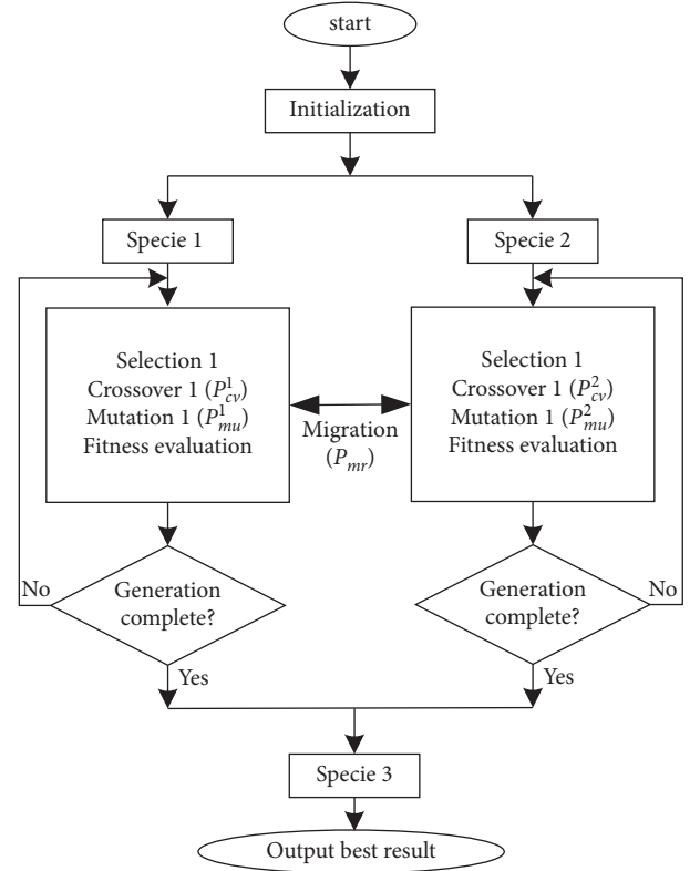
FIGURE 5: The layout of the proposed EGA with triple selection operation, self-tuning crossover operation, and three species.
