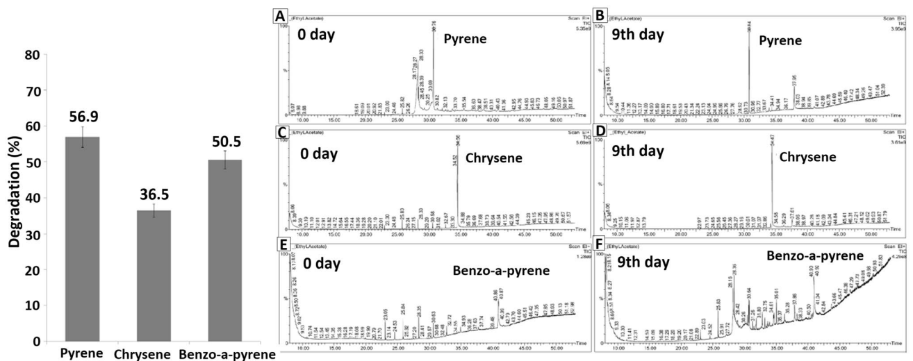
Fig. 5 Degradation (%) of pyrene, chrysene, and benzo(a)pyrene after 9 days of incubation by AWD5
