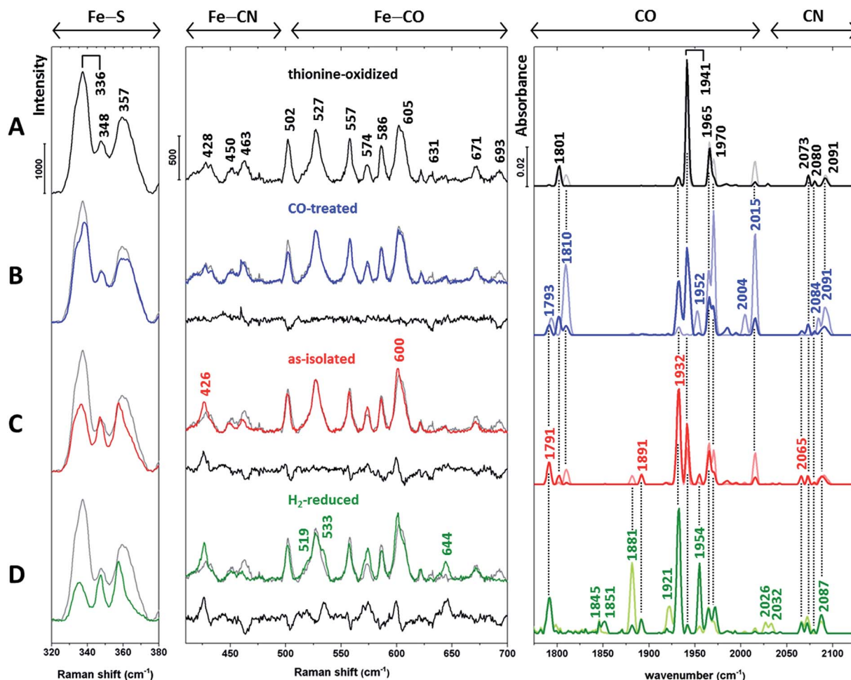
Fig. 3 Baseline-corrected vibrational spectra of (A) thionine-oxidized, (B) CO-treated, (C) as-isolated (dithionite-reduced), and (D) H 2 -reduced in vitro -matured holo-HydA1(adt). Low-temperature RR spectra (80 K, 488 nm excitation) are presented in two parts for the sake of clarity. The middle panel displays the spectral region reflecting Fe–CO/CN vibrations of the [FeFe] moiety, while the left panel is dominated by normal modes of the [4Fe4S] cluster. 11–16,22–25,28 The difference spectra in the middle panel (traces B–D, black lines) were calculated by subtracting the spectrum of thionine-oxidized holo-HydA1 (trace A, shown in grey) from coloured traces B–D prior to baseline-correction. RR spectra are normalized as described in the Experimental details section. Low-temperature IR spectra (80 K) of the CO and CN stretching modes of the [FeFe] moiety are depicted in the right panel (see Table 1 for band assignments). Lines in light and saturated colours represent spectra recorded in the dark and during blue light illumination (460 nm), respectively. Interestingly, IR spectra of H 2 -treated holo-HydA1(adt) exhibit a significant photo-induced decrease of the band at 1881 cm -1 and a concomitant absorbance increase at 1954 cm -1 (trace D). Previously, both bands were assigned to a single H sred state, 6 which appears unlikely according to this observation.
