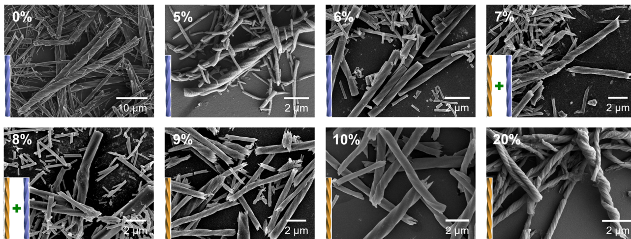
Fig. 2 SEM images of R-1H-x ( x = 0\text{--}20\% ) obtained via the hydrothermal reaction at pH 5.0 and 100 °C for 1 day.
